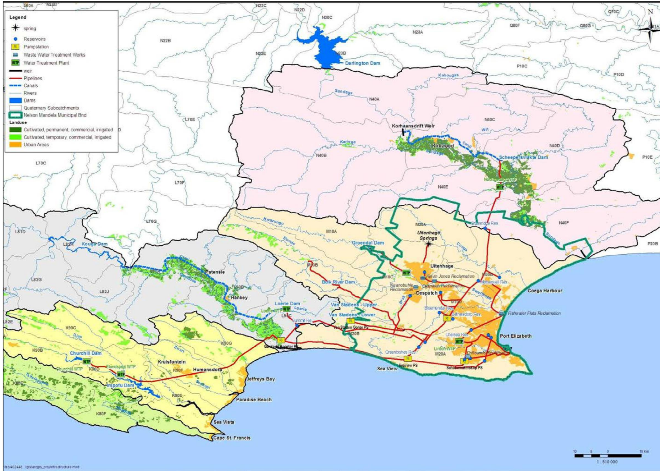
Figure 8-10: The Algoa Water Supply System
