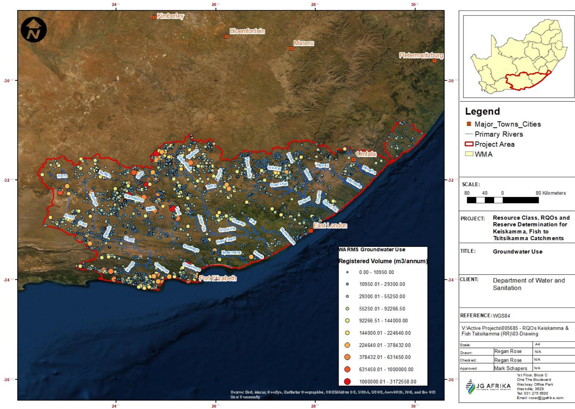
Figure 8-15: Groundwater use
