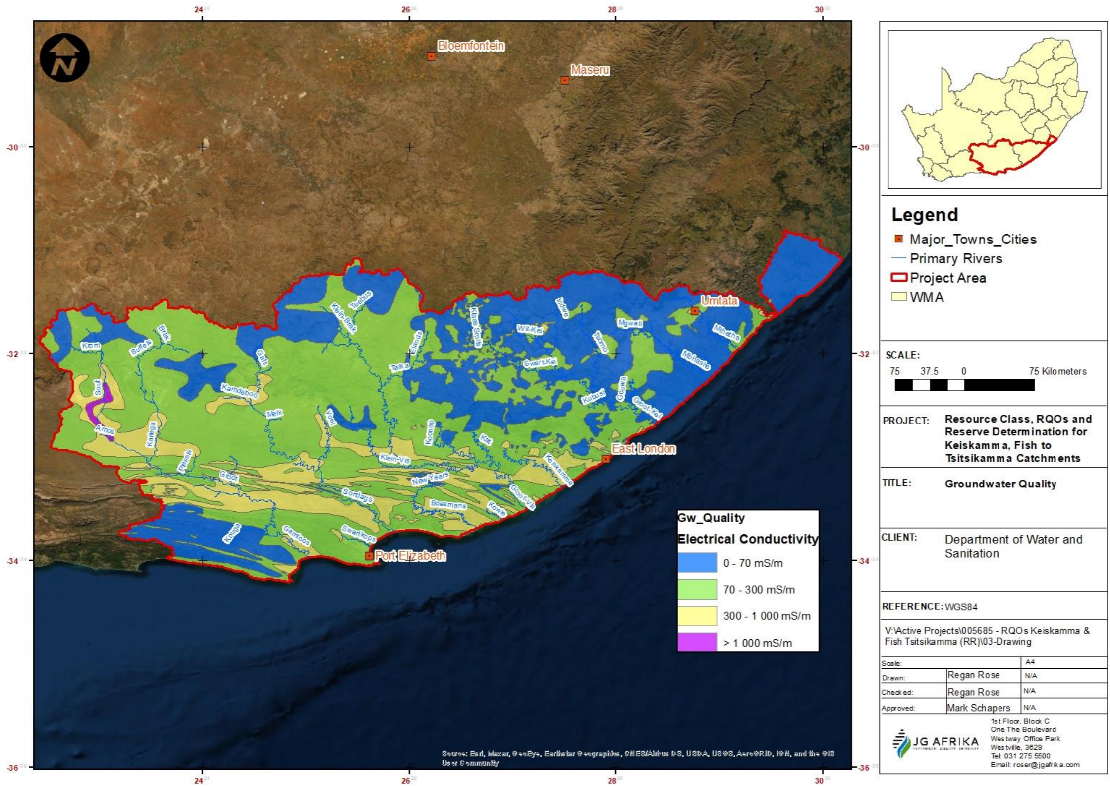
Figure 8-16: Groundwater quality
