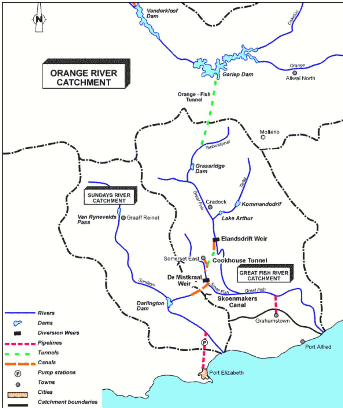
Figure 3-1: Infrastructure of the Fish-Sundays Transfer Scheme
