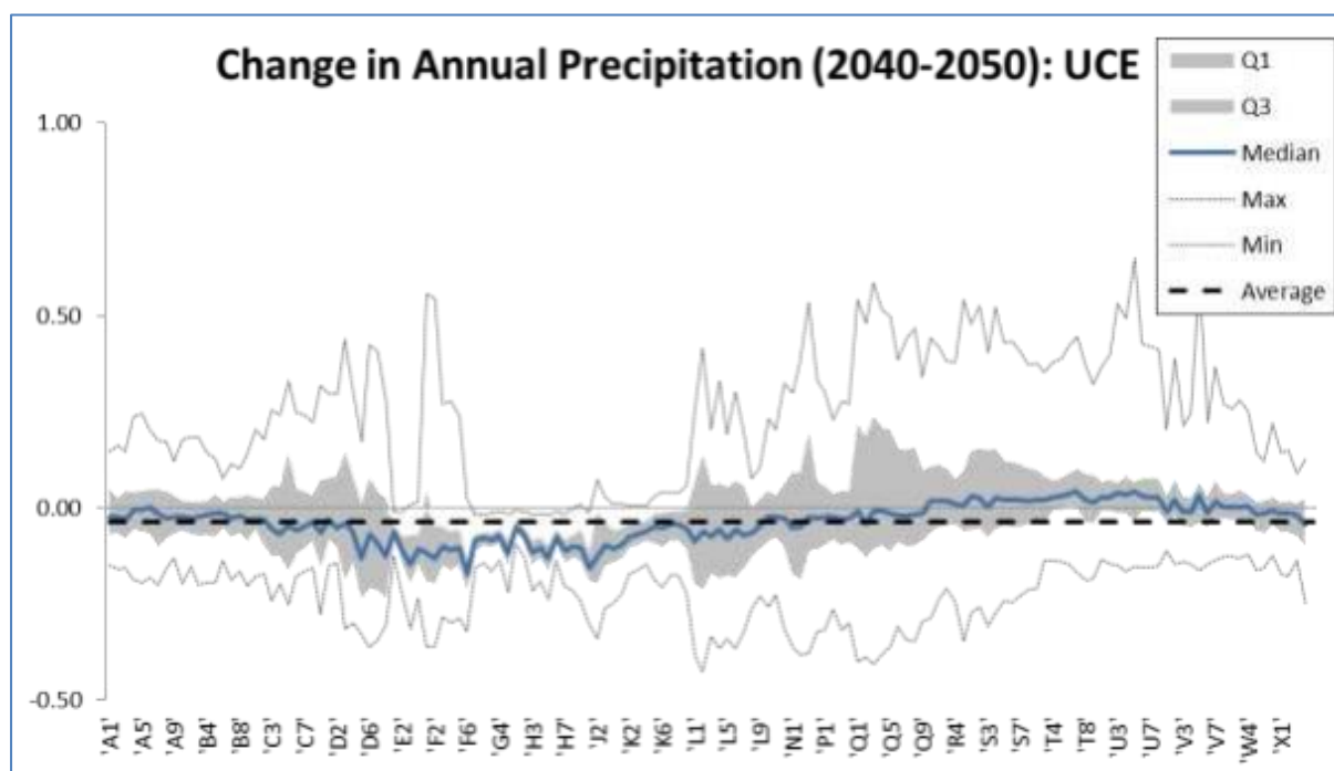
Figure 2-1: Projections of the possible impacts on precipitation of the UCE scenario
