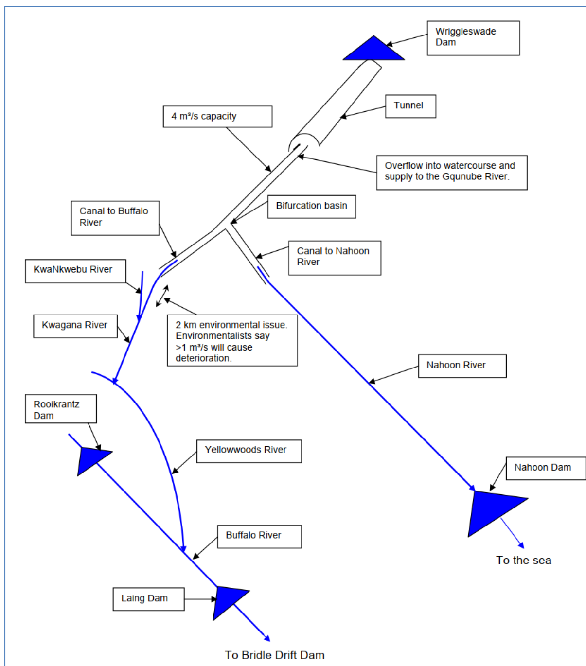
Figure 3-2: Key water resources infrastructure of the Amatola WSS
