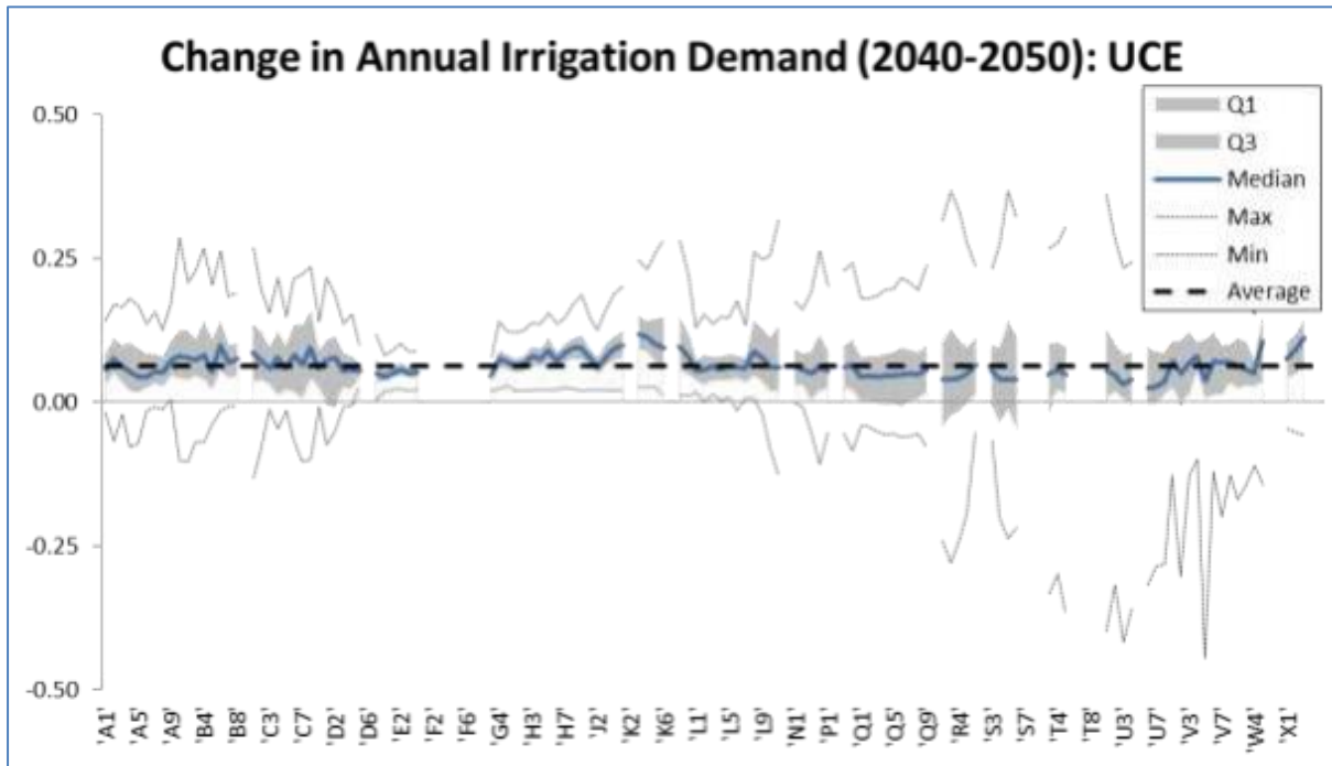
Figure 2-4: Projections of possible irrigation water requirement impacts for the UCE scenario
