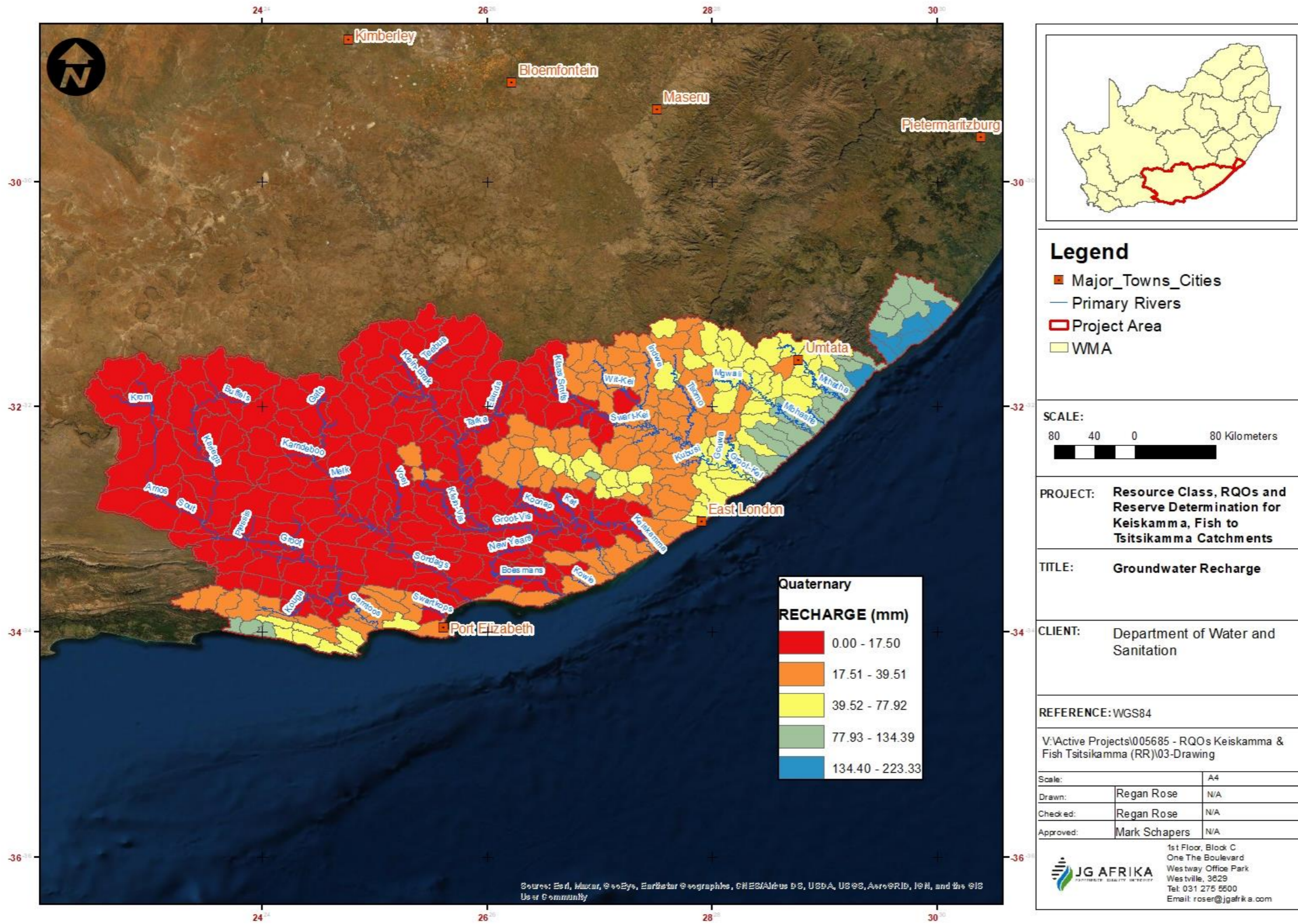
Figure 8-13: Groundwater recharge
