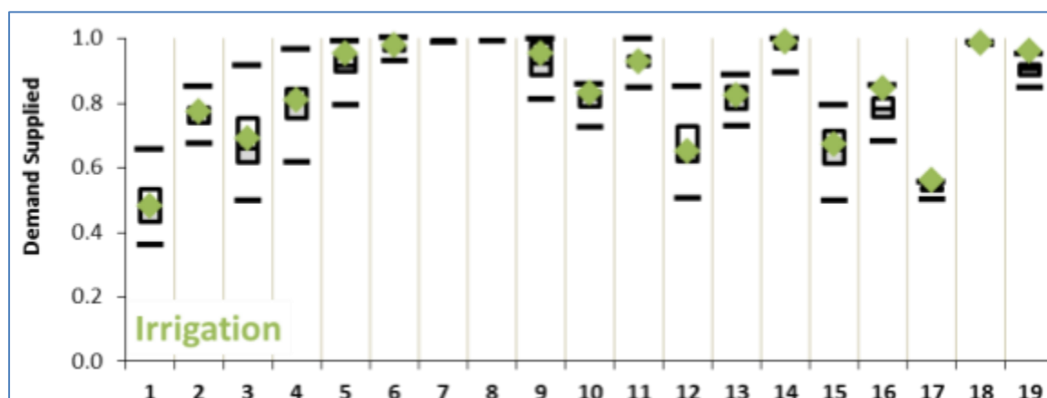
Figure 2-5: Projections of possible urban and irrigation water supply impacts in South Africa
