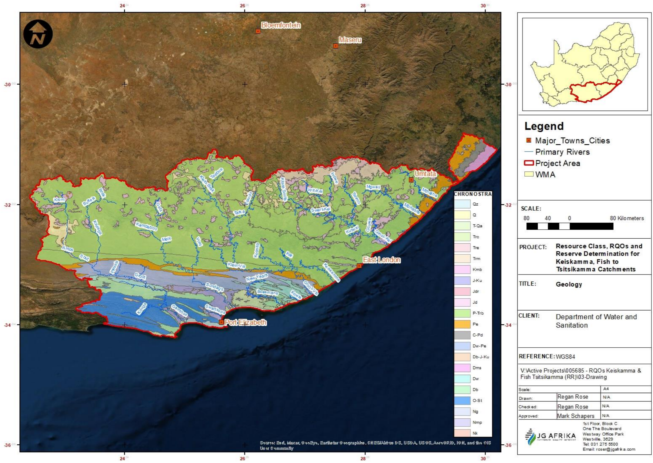
Figure 8-12: Geology
