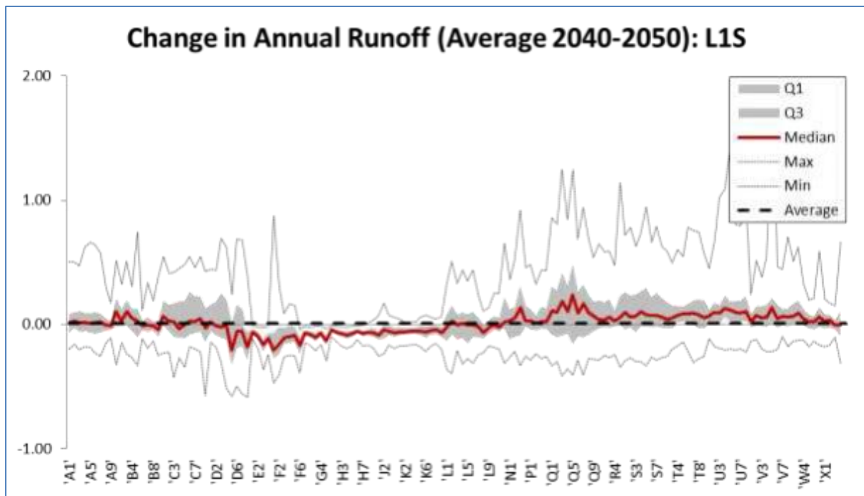
Figure 2-3: Projections of possible runoff impacts for the L1S scenario
