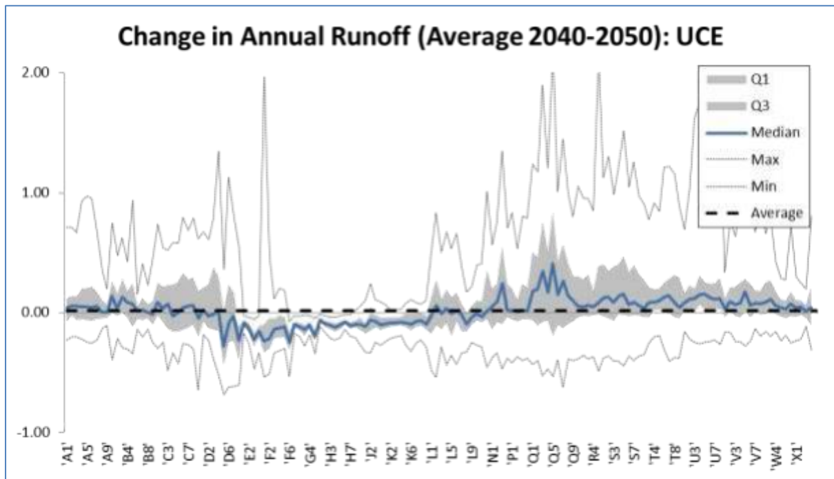
Figure 2-2: Projections of possible runoff impacts for the UCE scenario
